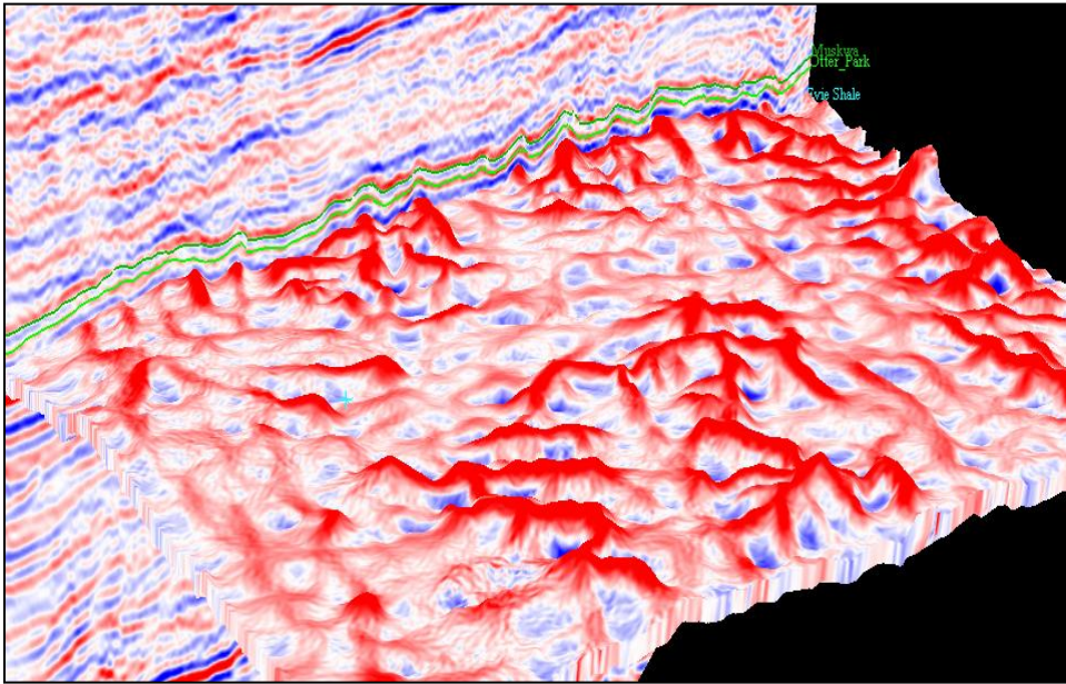
Figure 4: A horizon slice at the Muskwa level through the relative acoustic impedance volume derived from thin-bed reflectivity inversion of 3D seismic data co-rendered with most-positive curvature lineaments using transparency.
