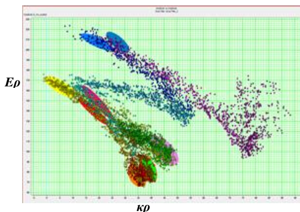
Figure 5b: Crossplot of \kappa\rho - E\rho with cluster covering the Ferni, Nordegg and the Montney formations. Clusters corresponding to these formations are seen much better separated than shown in Figure 5a.
