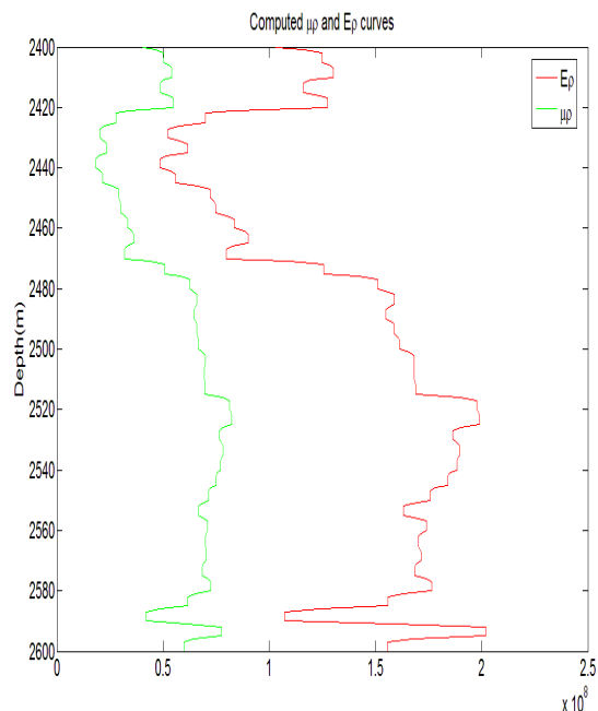
Figure 2: \mu\rho and E\rho curves computed from segmented input logs. On these segmented curves, more emphasized lithologic variation is seen on the E\rho curve than on the \mu\rho curve.
