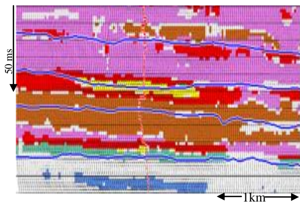
Figure 6a: Back projection of cluster points enclosed in polygons as seen in Figure 5a
