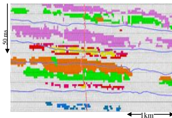
Figure 6b: Back projection of cluster points enclosed in polygons as seen in Figure 5b. It is noticed that upper and lower part of the Montney formation is distinguishable. Ferni and Nordegg formations are also seen as showing variation within their own zones.
