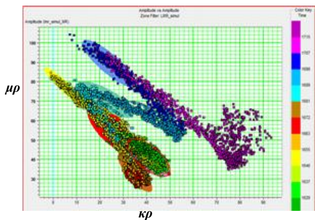
Figure 5a: Crossplot of \kappa\rho - \mu\rho with cluster covering the Ferni, Nordegg and the Montney formations. Clusters corresponding to these formations are seen separated.
